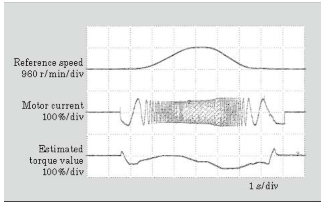
Fig.2 Characteristics of elevator operation by torque vector Table 2 Applicable encoder interfaces control (without a speed sensor)
