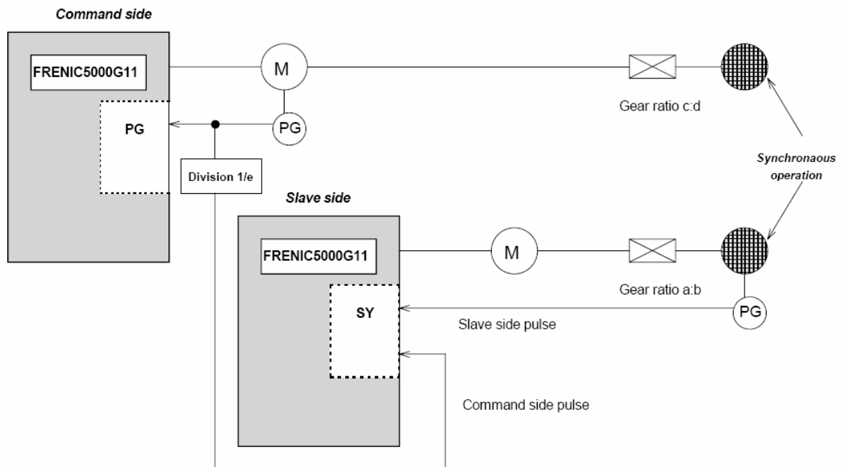
Figure 4. Example system setup.
