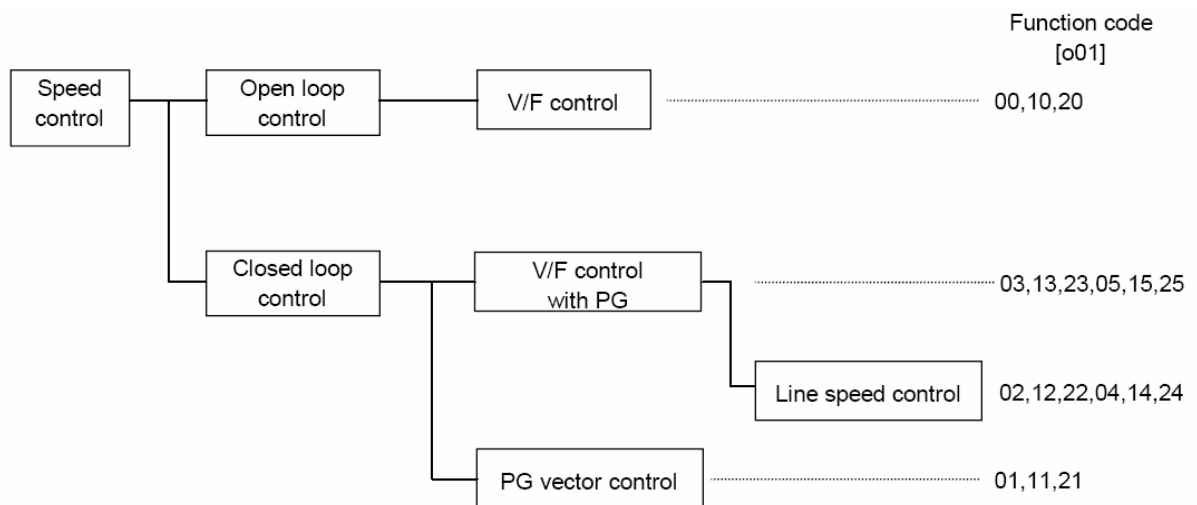
Figure 1. Different alternatives for speed control.
