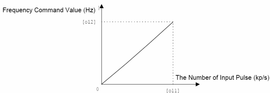
Figure 2. Relationship between pulse input frequency and frequency command.
