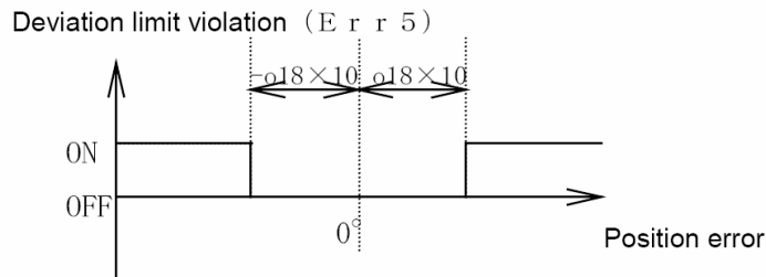
Figure 3. Deviation limit violation error.
