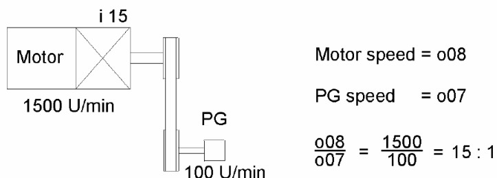
Figure. Example of setup with closed loop operation.
